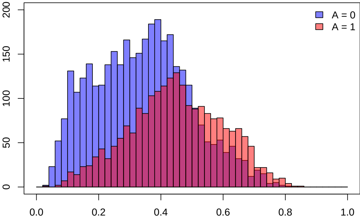
Propensity Score Overlap
